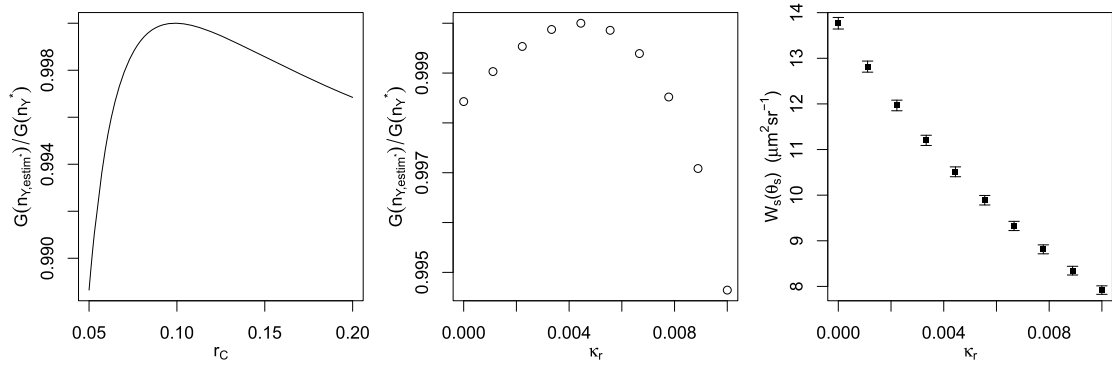
Fig. 1. Test case described in Sec. 3. Left panel: ratio of the obtained efficiency gain G(n_{Y,estim}^*) (where n_{Y,estim}^* was computed using the estimated value r_{C,estim} = 0.1 ) to the maximal possible efficiency gain G(n_Y^*) (obtained with the exact value r_C ) as function of r_C . Mid panel: ratio of the obtained efficiency gain G(n_{Y,estim}^*) (where n_{Y,estim}^* = 8 \cdot 10^3 was computed for \kappa_r = 4 \cdot 10^{-3} ) to the maximal possible efficiency gain G(n_Y^*) (obtained with the value n_Y^* corresponding to \kappa_r ) as function of \kappa_r . Right panel: differential scattering cross section W_s(\theta_s) as function of \kappa_r (for n = 2 \cdot 10^4 ). Error bars indicate the Monte Carlo standard error \sigma_A . The used parameter values are \theta_s = 0.244 , \bar{R} = 0.5 , s_R = 1.2 , \bar{r}_{eq} = 2.38 \mu\text{m} , s = 1.18 , k_e = 14.0 \mu\text{m}^{-1} , n_r = 1.08 and, for the left panel, \kappa_r = 4.10^{-3} .
